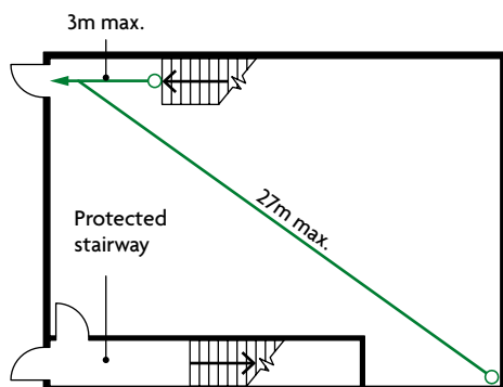
Ground storey
