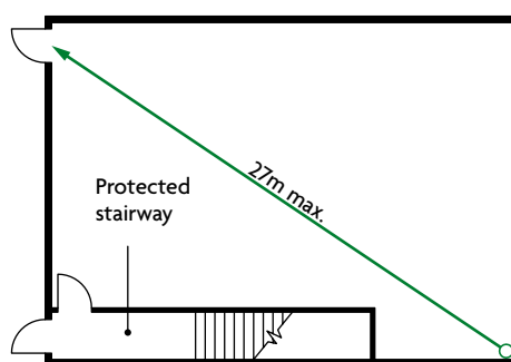
Ground storey
