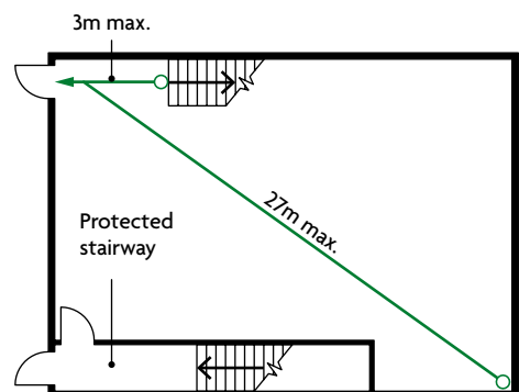
Ground storey
