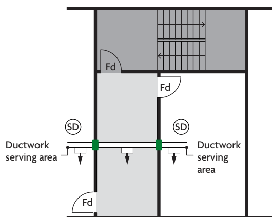
Diagram 10.3 Ductwork passing through protected escape routes – method 4
