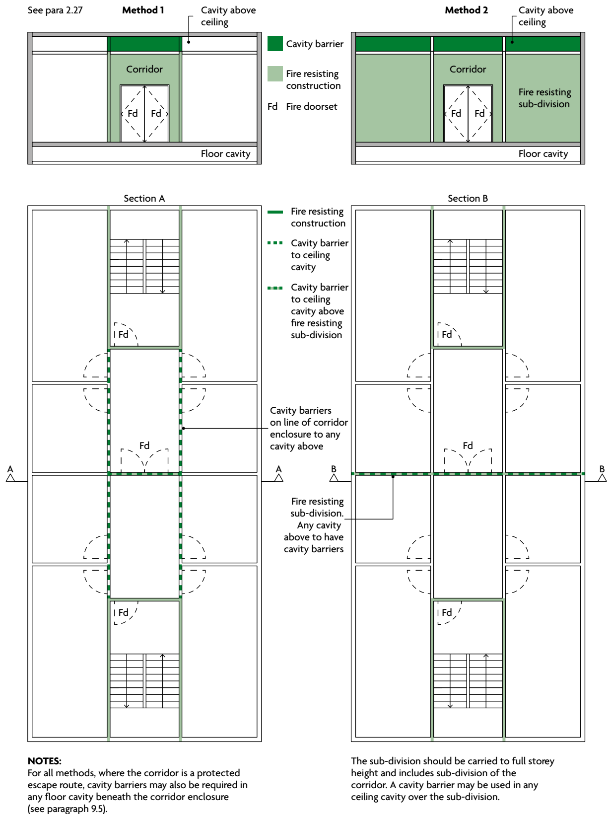
Diagram 2.9 Division of corridors
